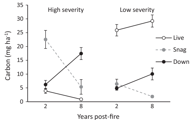
Fig. 3. Carbon ( Mg\ ha^{-1} ; \pm 1\ SE ) measured in three pools 2 years and 8 years post-fire, combined across treatments in high-severity and low-severity burn areas.
