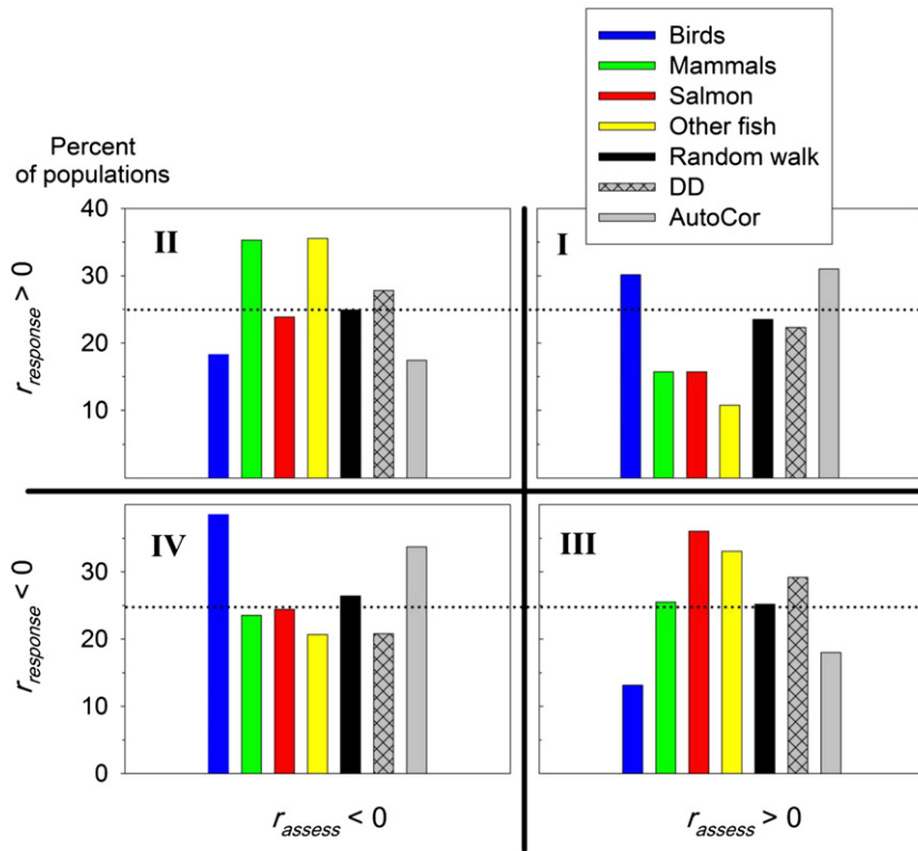
Fig. 2. Percent of populations of each of the major taxonomic groups that fall into each of four quadrants (I–IV), defined by the relationship between r_{response} and r_{assess} . Percentages are calculated over the sample sizes shown in Table 1. The dotted line at 25% is the expected result for populations whose time series of abundance represents a random walk, such that growth rate at time t + 1 is independent of growth rate in previous time periods. Black and gray bars show results for data simulated under three different null models, using the following parameters: Random walk ( \sigma = 0.02 ), AutoCor (random walk with lag-1 temporal autocorrelation; \sigma = 0.02, \rho = 0.9 ), and DD (density dependence with random fluctuations in carrying capacity; R_0 = 1.5, K varied randomly in range 600–1000).
