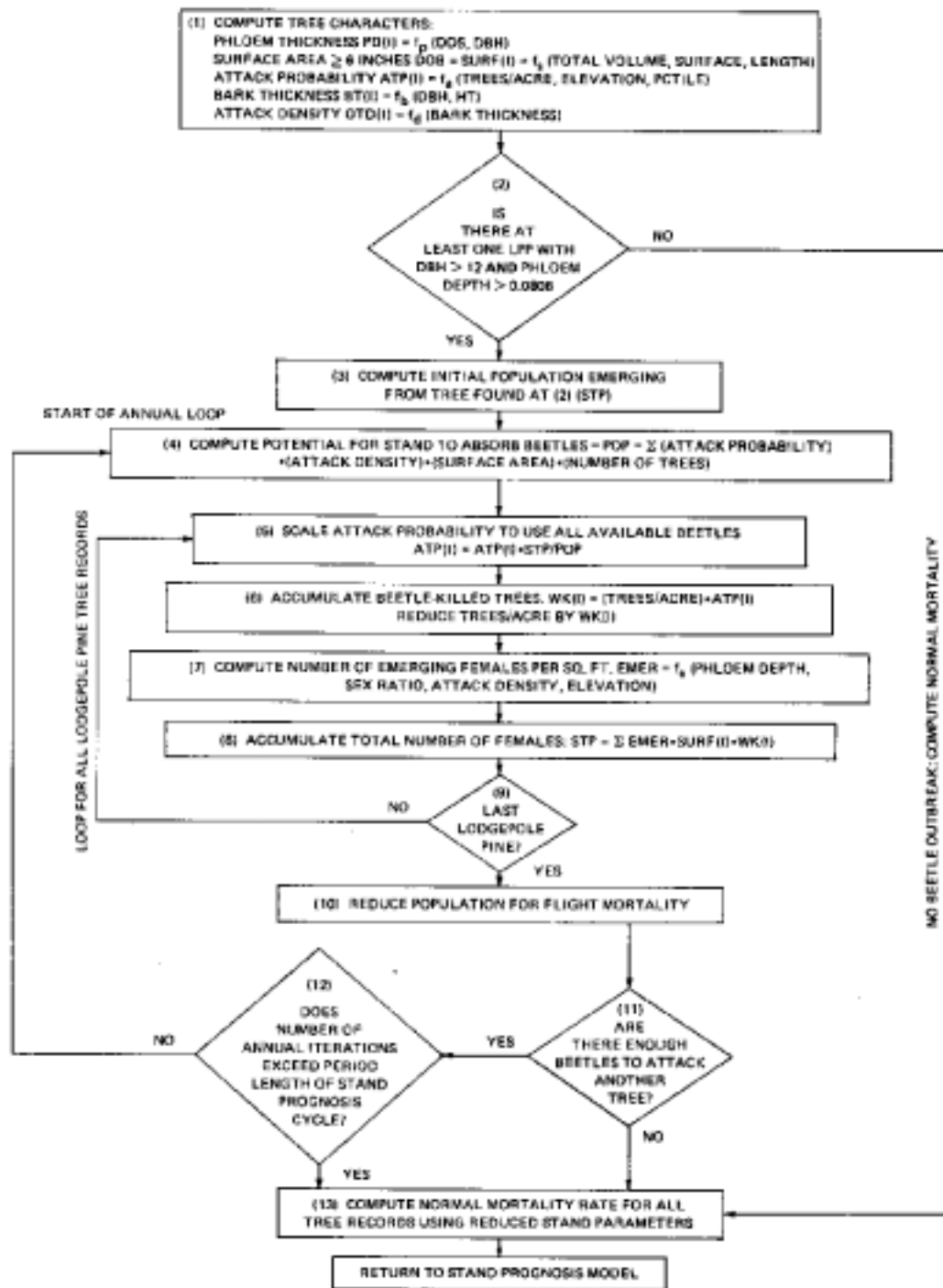
Figure 3.--Logic flow of subroutine for mountain pine beetle impact.
