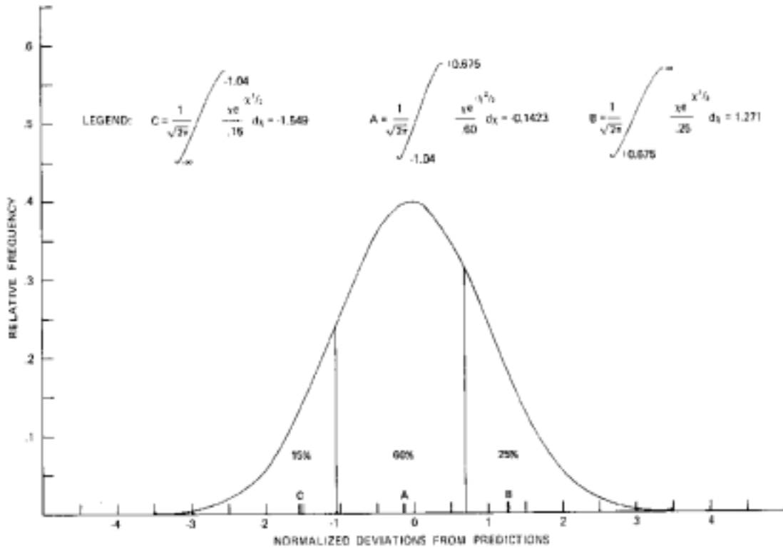
Figure 2.--Location of prediction points for three fractions of Normal Distribution.
