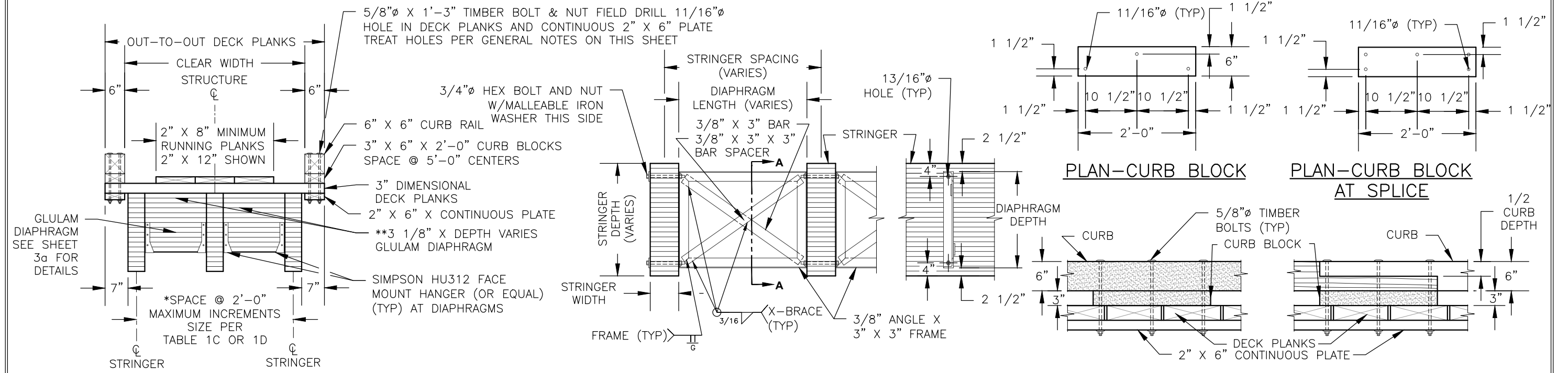
BRIDGE W/RAILING SYSTEMS DECK SECTION W/STRINGERS @ 2'-0" O.C.
