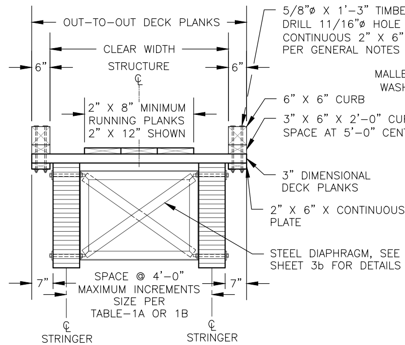
BRIDGE W/CURBS ONLY DECK SECTION W/STRINGERS @ 4'-0" O.C.
