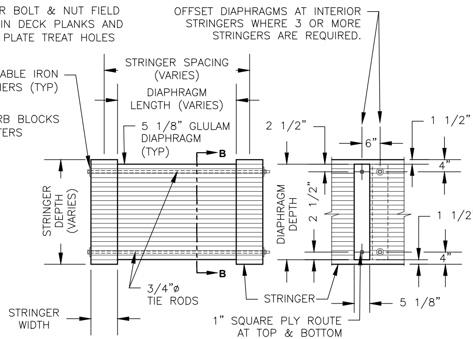
ELEVATION-SECTION B-B GLULAM DIAPHRAGM ALTERNATE GLULAM DIAPHRAGM ALTERNATE IS APPLICABLE FOR ALL STRINGER DEPTHS.
