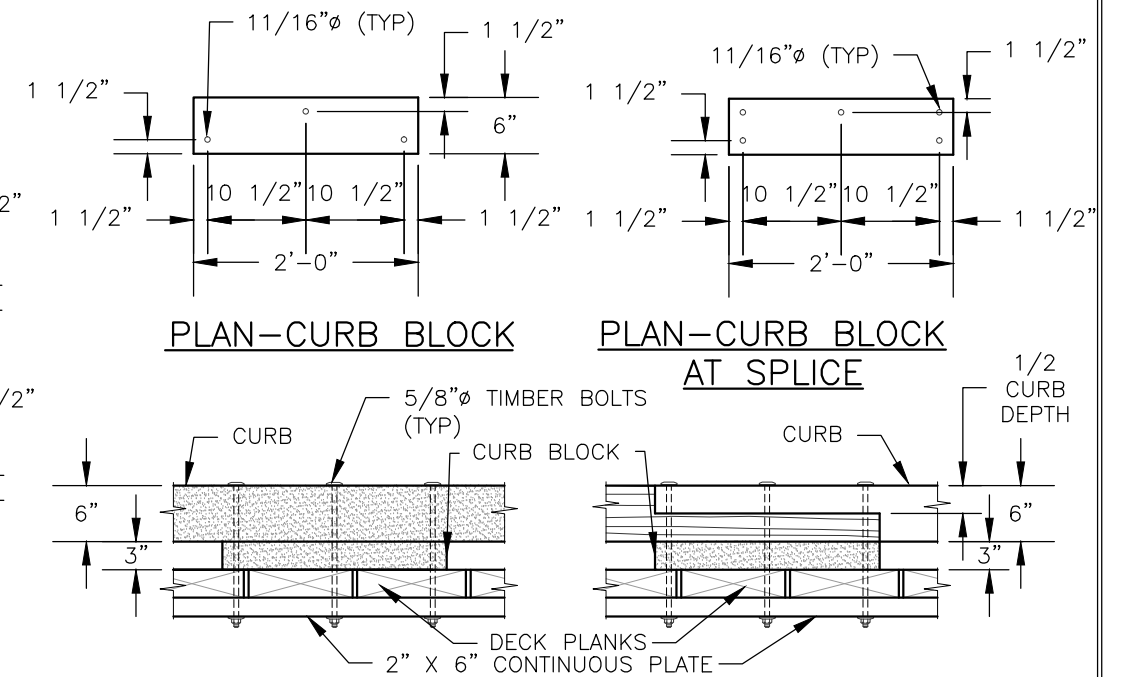
ELEVATION-TYPICAL CONNECTION ELEVATION-CONNECTION AT SPLICE SOLID SAWN CURB CONNECTION DETAILS
