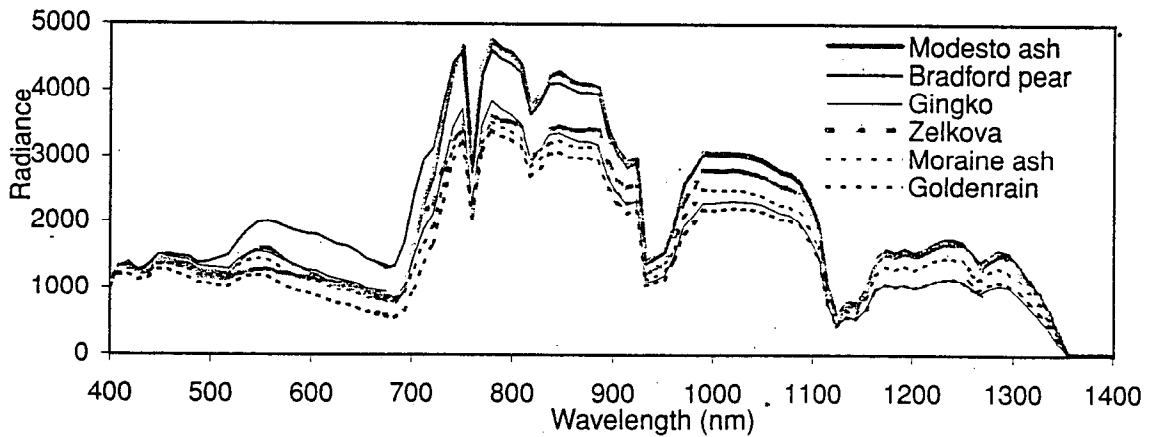
Figure 7. Radiance of different broadleaf deciduous tree species. Modesto ash and bradford pear have higher radiance in the infrared wavelength region. Bradford pear has highest radiance in the visible region; Goldenrain has lowest radiance.
