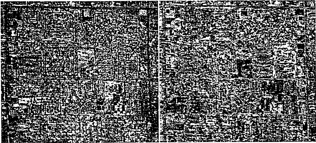
c. Broadleaf evergreen d. Conifer
