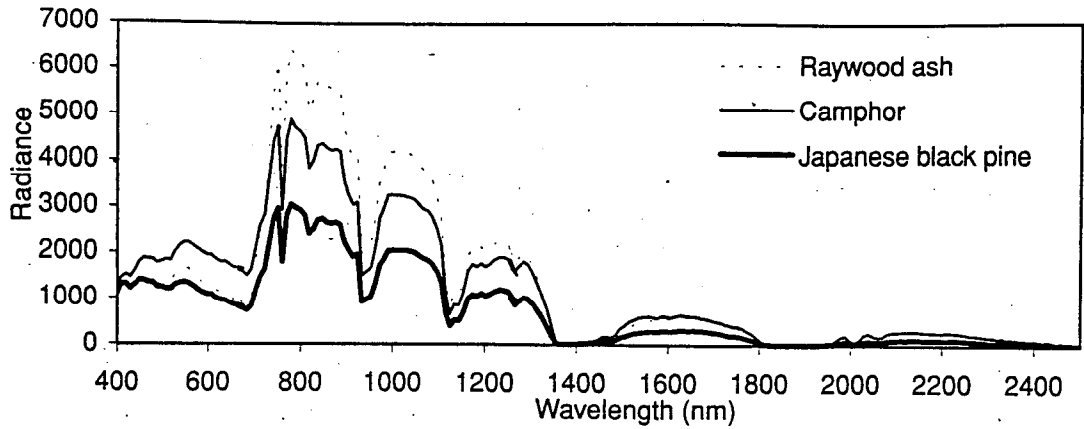
Figure 6. Radiance of three tree types. Japanese black pine (conifer) has lowest radiance. Raywood ash (broadleaf deciduous) has highest radiance in the infrared region. Camphor (broadleaf evergreen) has radiance between the other two trees, but it has highest radiance in visible wavelength region.
