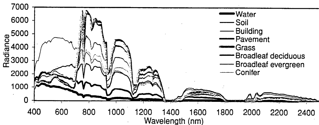
Figure 8. Radiance of endmembers. Radiance for eight endmembers are shown in this figure. The radiance of these ground properties not only varies with magnitude but also the spectral patterns are different.
