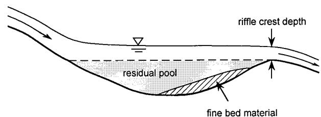
Figure 2. Definition sketch of V^* . In this longitudinal profile the residual pool volume extends from the coarse substrate (heavy line) to the elevation of the riffle crest (dashed line).
