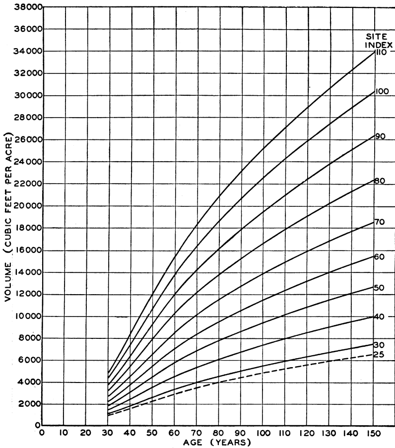
FIGURE 6.—The volumes in cubic feet (inside bark, stump and top included, for average well-stocked stands of average composition
