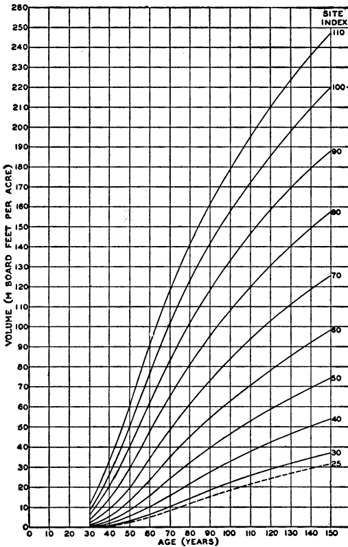
FIGURE 8.—Volume in board feet by the international rule (1/8-inch kerf), trees 8 inches and larger, average of well-stocked stands, average composition.
