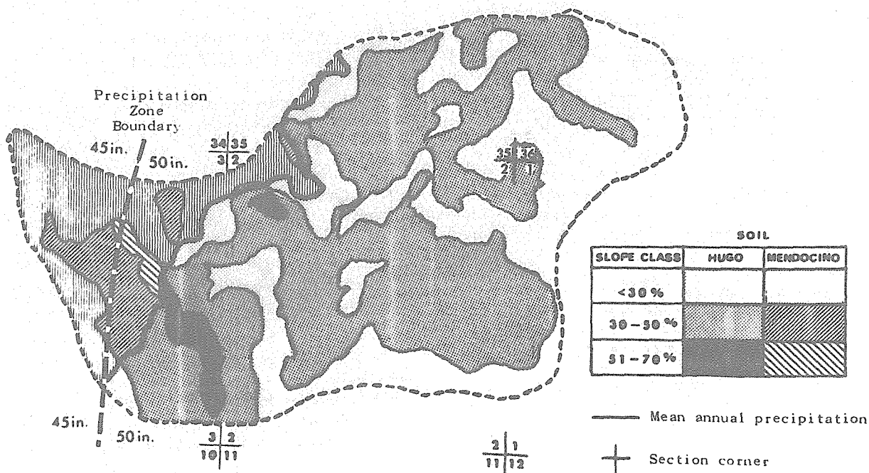
Figure 1—Homogeneous soil and slope classes were mapped as shown here for the north fork of Caspar Creek.
