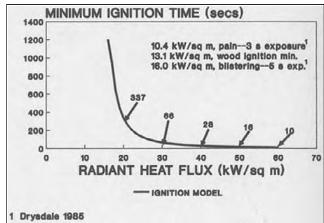
Figure 7 —Minimum ignition time vs. radiant heat flux. Given a constant radiant heat flux, the ignition model (SIAM) can be used to estimate the time required for sustained ignition on a flat wood surface. The references to pain and blistering relate to exposed skin at the given radiant heat fluxes.
