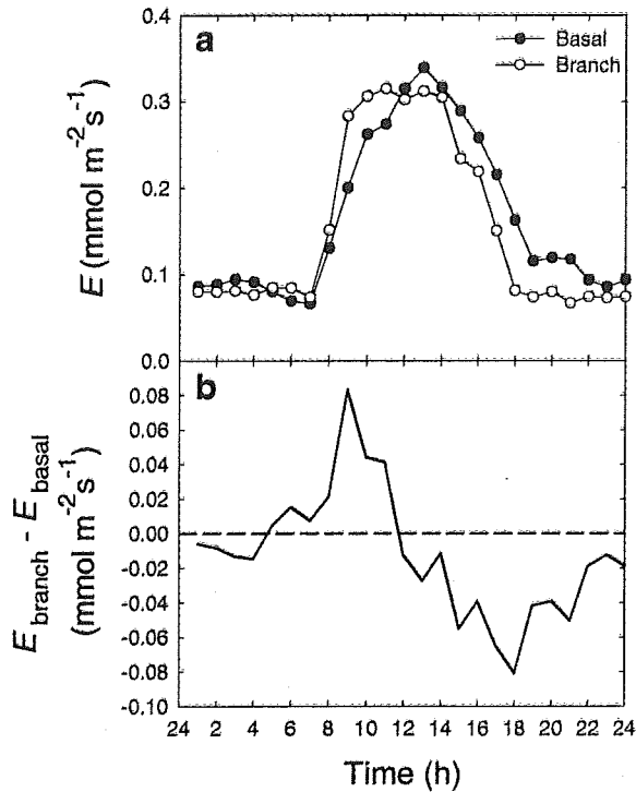
Fig. 2 a Representative daily courses of transpiration ( E ) estimated from terminal branch sapflow ( open circles ) and from basal sapflow ( closed circles ) measured with heat pulse probes. b Difference between branch and basal transpiration on the same day (August 24, 2004) as in panel a, in one individual of Ouratea hexasperma , a dominant woody species with low leaf area index of Cerrado savanna in central Brazil. Positive values indicate time periods when a fraction of transpired water was withdrawn from internal water storage, and negative values indicate time periods when water from the soil was refilling stem storage. Heat pulse systems (single point sensors) were placed at the same depth below the cambium at the base (6.1 cm basal diameter) and in a terminal branch (3.1 \text{cm}^2 sapwood area). Transpiration was obtained by dividing volumetric sap flow by the total leaf area per plant or per branch
