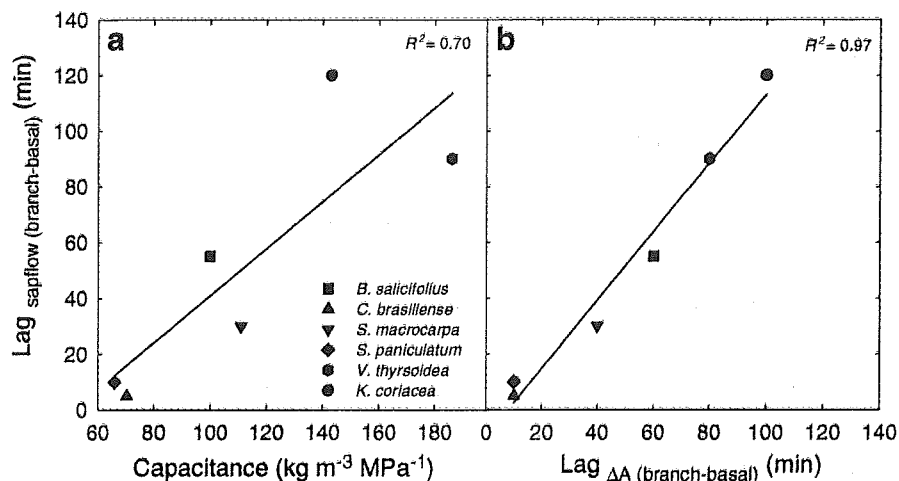
Fig. 3 The time series lag (i.e. lag corresponding to maximum correlation between time series) between branch and basal sap flow ( \text{Lag}_{\text{sapflow (branch-basal)}} ) in relation to a total stem capacitance (sapwood and outer parenchyma) and b the time series lag between branch and trunk cross-sectional area ( \text{Lag}_{\Delta A \text{ (branch-basal)}} ) for six dominant woody species of ~ Neotropical savannas. Branch and bole sap flow were measured with thermal dissipation probes and branch and bole cross sectional areas ( \Delta A ) were calculated from diameter measurements using electronic dendrometers (data from Scholz et al,
