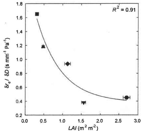
Fig. 4 – Canopy resistance per unit change in vapor pressure deficit ( \delta r_c / \delta D ) as a function of annual mean LAI for all physiognomies along the gradient. The line is an exponential decay function fitted to the data y = 0.4 + 1.9 \exp(-1.5x) , P < 0.1 . \delta r_c / \delta D is the slope of the linear relationships obtained between r_c and D as shown in Fig. 3. Symbols as in Fig. 3.
