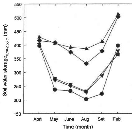
Fig. 6 – Seasonal variation in soil water storage in the 0.10–2.50 m layer in five physiognomies along the gradient. Symbols as in Fig. 3.
