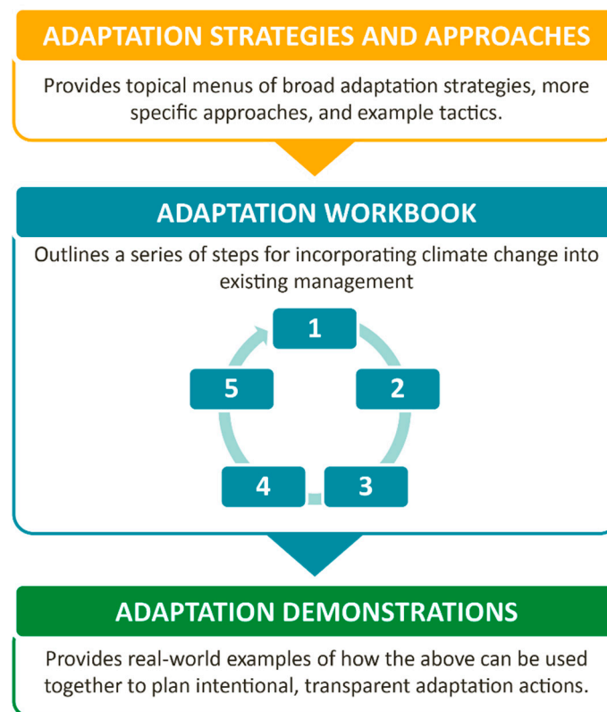
Figure 1. Adaptation tools within the CCRF. Figure reproduced with permission [10].
