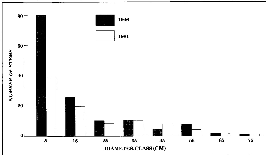
Figure 4. — D.b.h. class distribution for laurel sabino ( Magnolia splendens Urban) in 1946 and 1981 on permanent plots totaling 3.2 ha in the colorado forest. D.b.h. classes are: 5 cm (4.1 - 9.9 cm); 15 cm (10.0 - 19.9 cm); and in 10-cm increments through 75 cm (70.0 - 79.9 cm).
