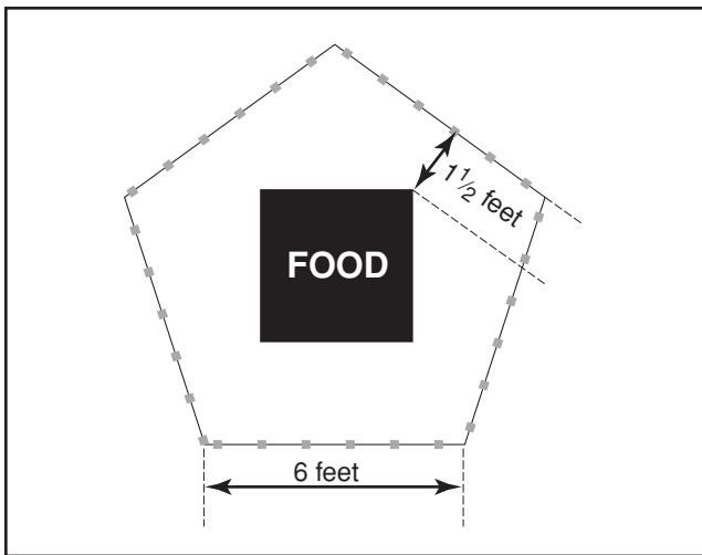
Figure 4—A recommended fence enclosure for backpacker’s food would have five 6-foot-long sides. Food must be stored at least 1½ feet away from the fence. Outfitters needing to protect more food can combine two of these fences to enclose an area with 12-foot-long sides.
