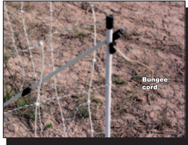
Figure 6—Bungee cords can be used to hold diagonal braces against corner posts.
