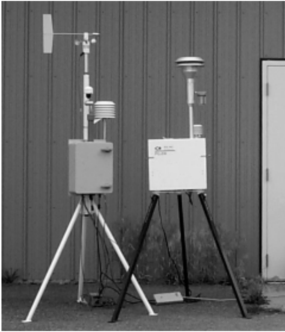
Figure 16—Instrument layout at the Bitterroot National Forest supervisor's office in Hamilton, MT.
