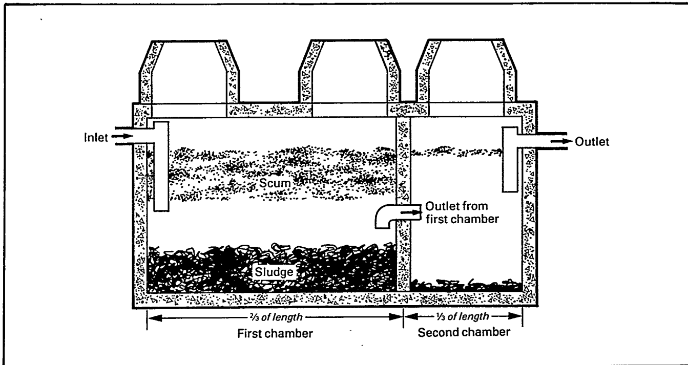
Figure 2. Typical septic tanks (continued).
