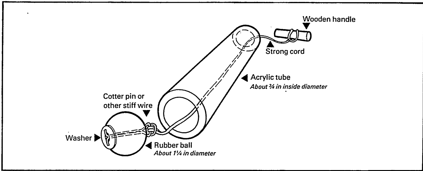
Figure 10. Scum/sludge layers measuring tube.
