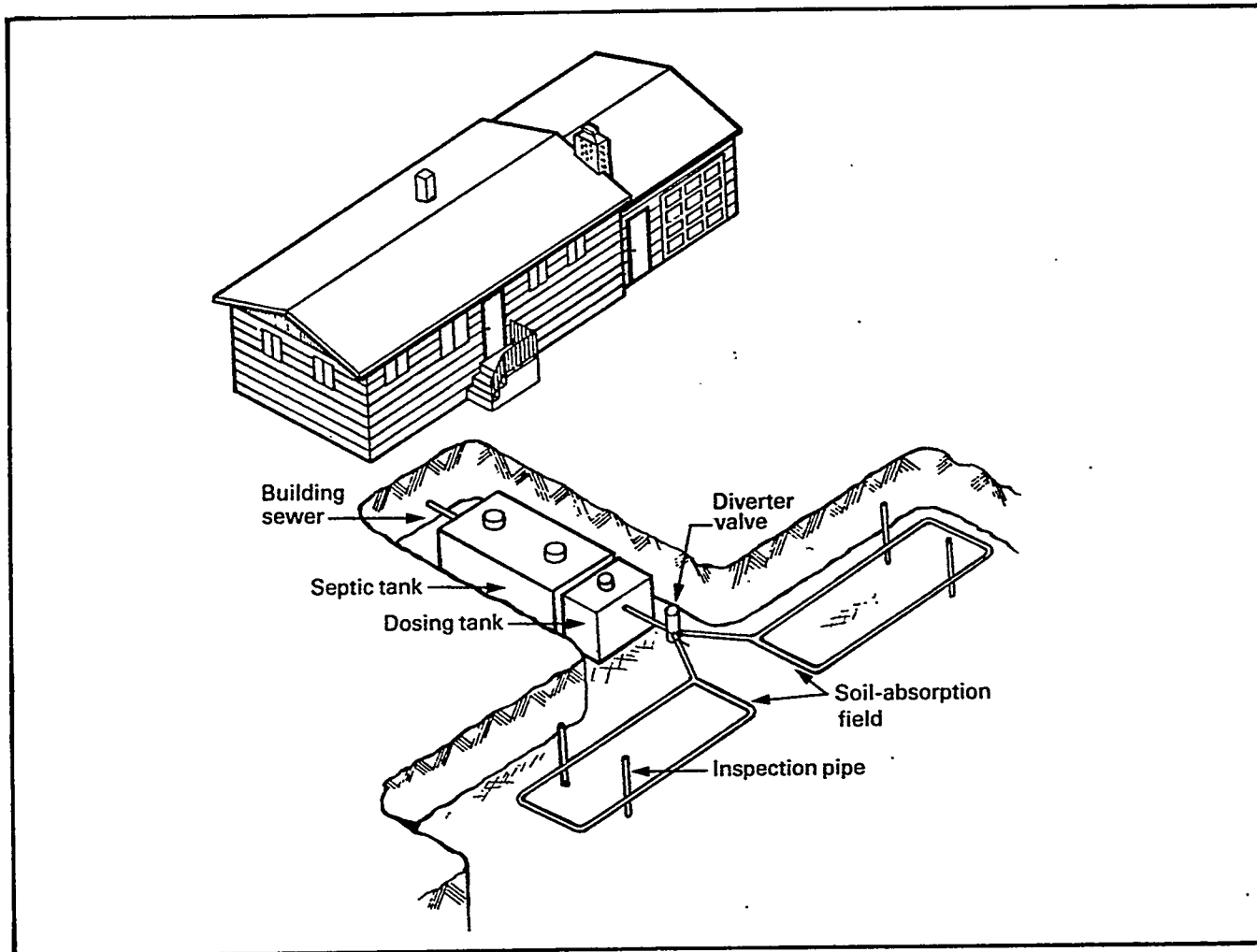
Figure 1. Typical ST/SAS.
