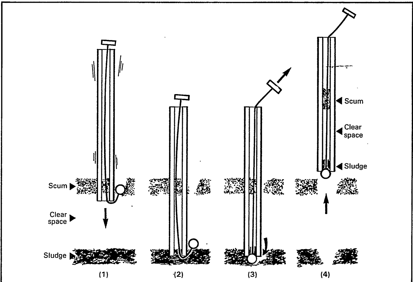
Figure 11. Use of measuring tube.
