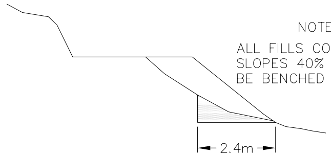
BENCHING TYPICAL NO SCALE
