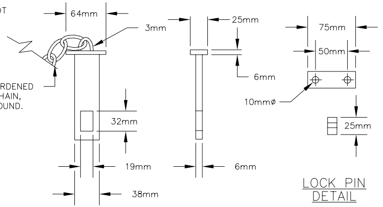
MASTER PIN DETAIL
