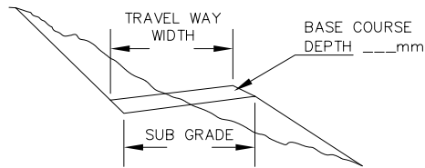
IN SLOPE SUB GRADE W/O DITCH, ____ %
