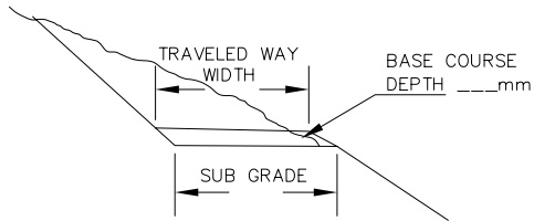
OUTSLOPE SUB GRADE W/O DITCH, ____ %
