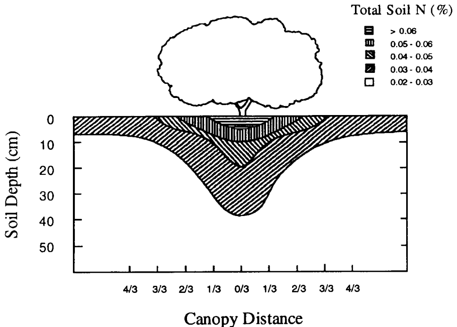
Figure 2. Nutrient isolines for total N% beneath isolated tree within a desert ecosystem in the south-western USA. Source: Klemmedson and Barth (1975).
