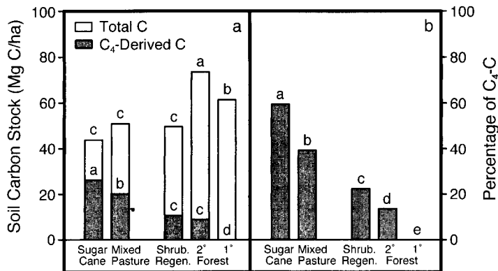
FIG. 2. (a) Total soil C and C 4 -derived C stocks and (b) proportion of C 4 -C beneath sugar cane, traditional pasture, successional vegetation, and old-growth forest (0–15 cm soil depth). The C 4 -derived soil C stocks of secondary vegetation were based on sugar cane values and were equal to values based on traditional pasture values. Data from two replicate sites are combined within each land-use type. The same letter above bars indicates that total soil C and C 4 -C stocks and the proportion of C 4 -C do not differ using Tukey's means comparison test (0.05 critical value).
