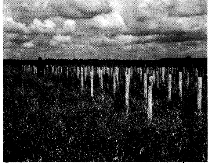
Figure 4.-The plot in the more humid area near Brookings, South Dakota, has a silt loam soil with pH of 6.3. Normal annual precipitation averages about 22 inches and annual temperature about 42°F.
