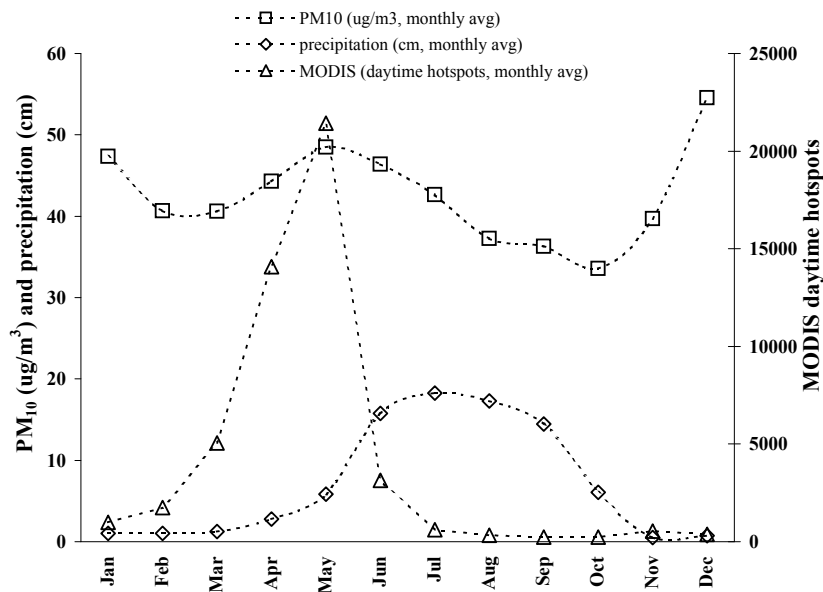
Fig. 6. Time series of monthly average PM 10 (Pedregal RAMA station 2003–2008 average, www.sma.df.gov.mx/simat/cambia_base.htm ); MODIS daytime hotspots for Mexico (2003–2008 average, www.conabio.gob.mx ); and monthly average precipitation for MCMA (see Sect. 4.2).
