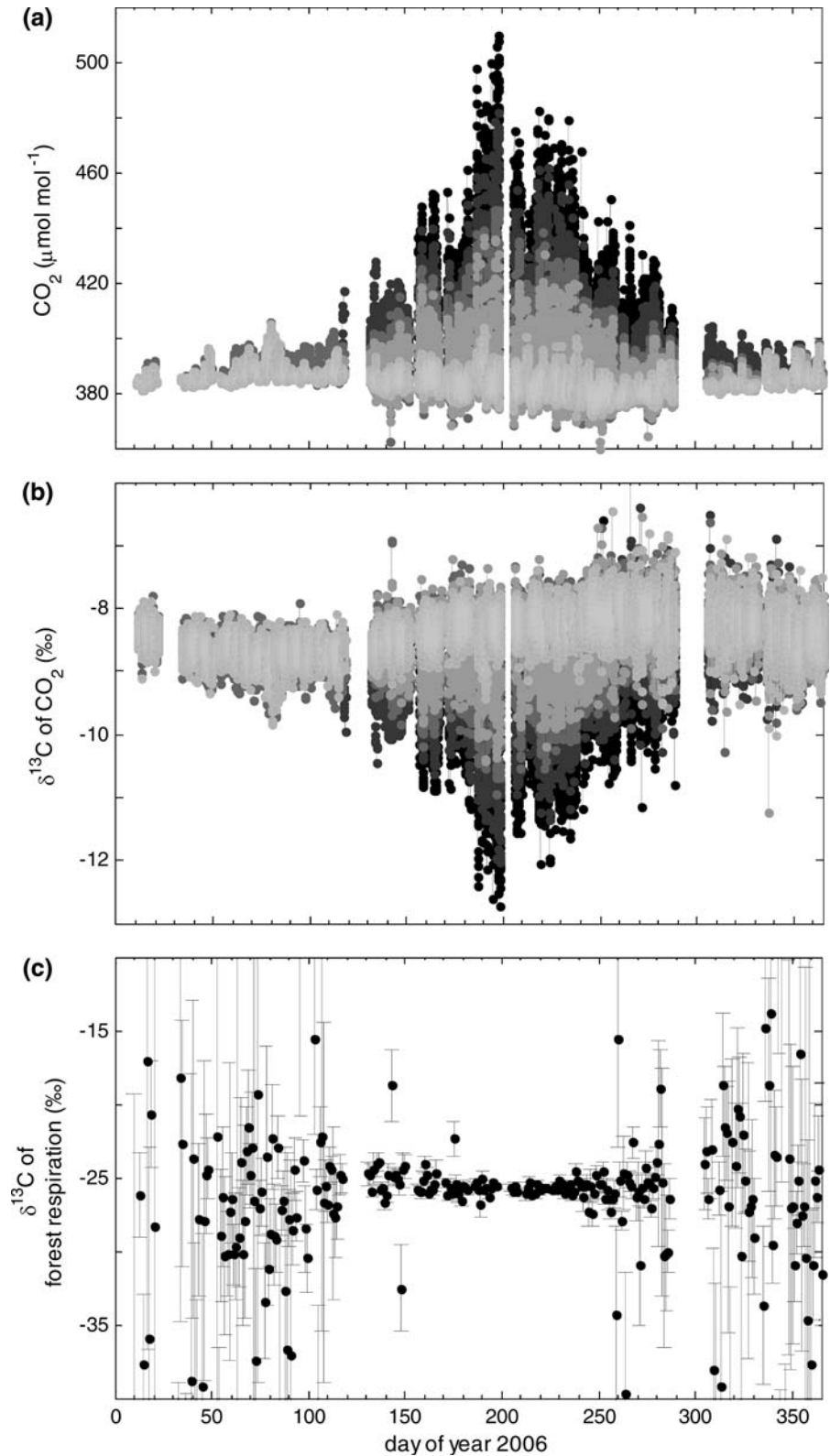
Fig. 1 (a) \text{CO}_2 and (b) \delta^{13}\text{C} of \text{CO}_2 in forest air at several heights (0.1, 1, 5, 7, 21.5 m) during 2006.
