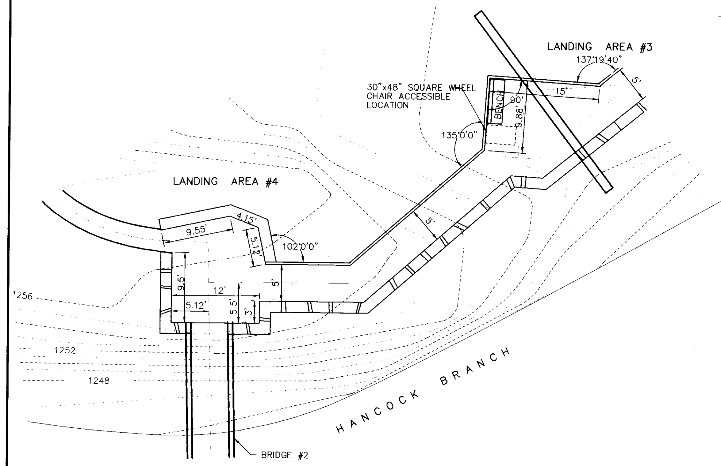
LANDING AREAS #3 & #4 1/8" = 1'-0"
