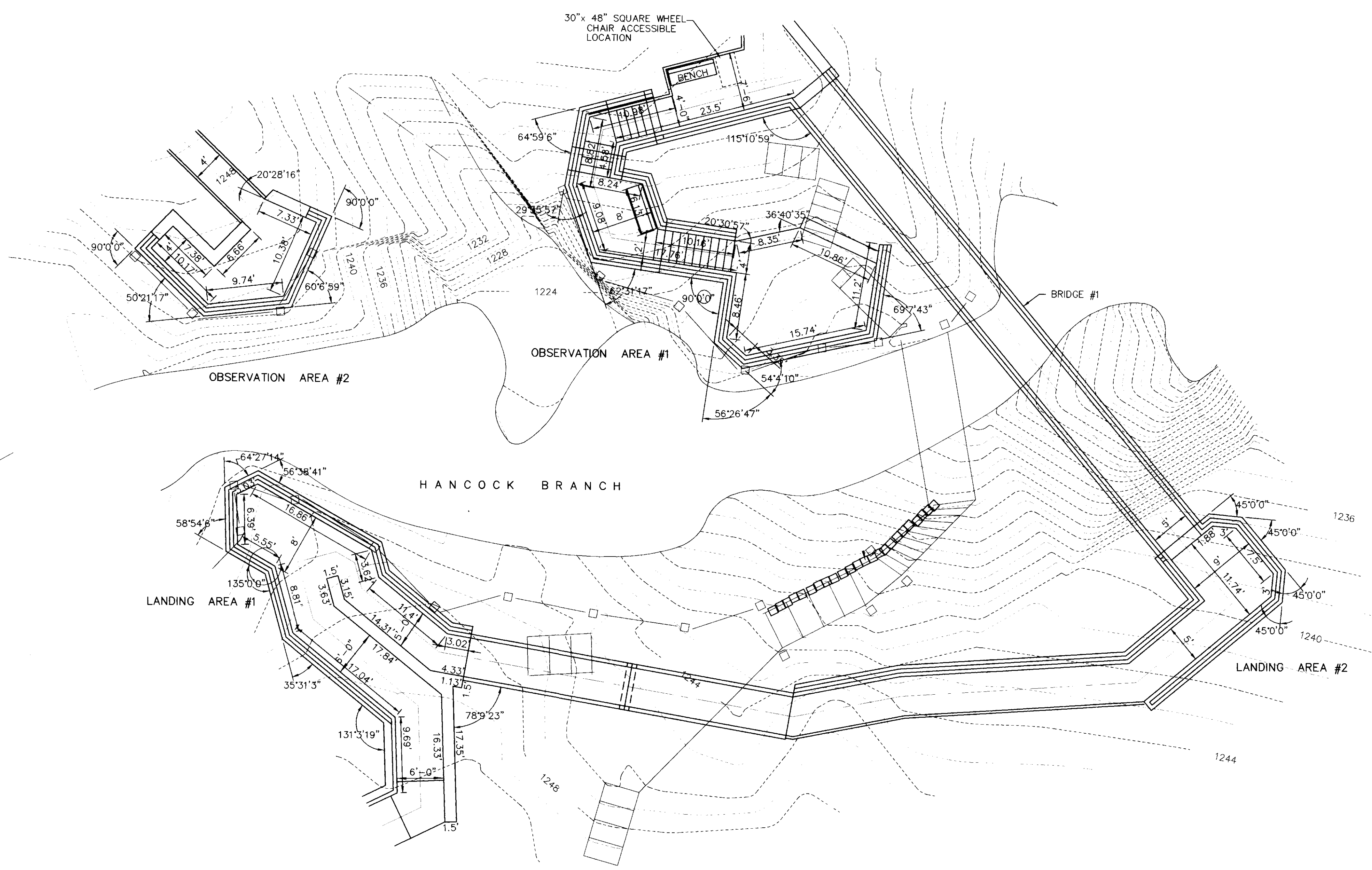
LANDING AREAS #1 & #2 & OBSERVATION AREAS #1 & #2 1/8" = 1'-0"
