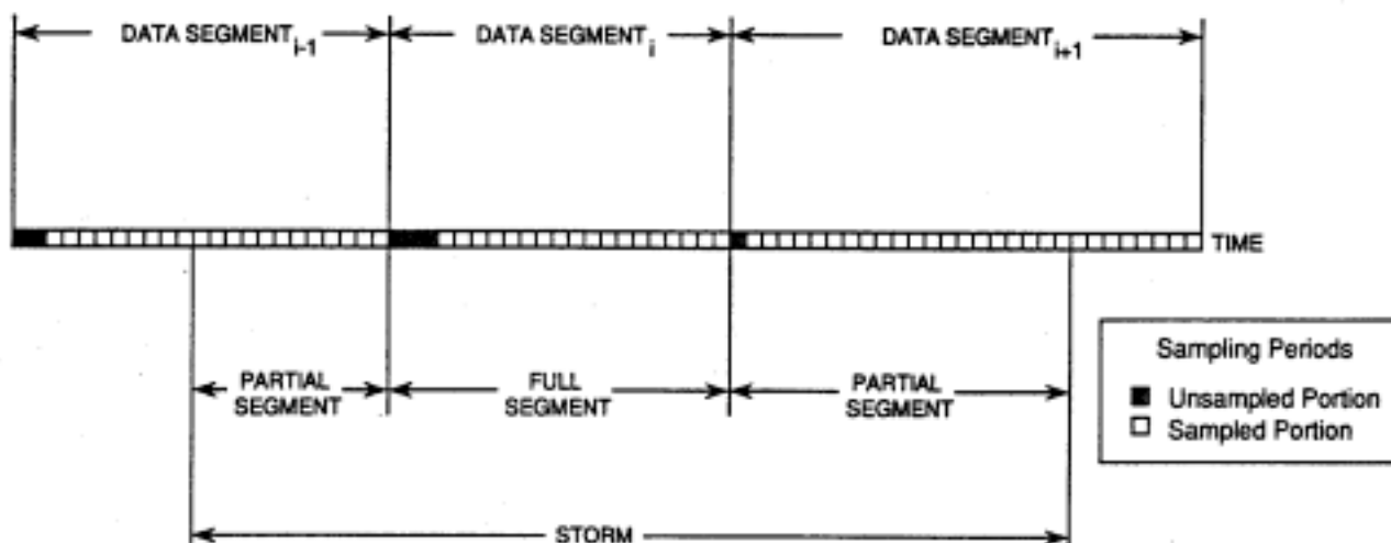
Figure 1 -Typical Piecewise SALT (Selection At List Time) time diagram. Data segments (time between station visits) contain integral numbers of sampling periods. Several sampling periods heading each segment are called the unsampled portion because the SALT program is idle for station
