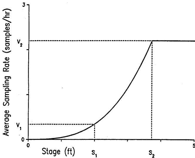
Figure 3 -Average sampling rate curve. Two design stages s_1 and s_2 and their corresponding average sampling rates v_1 and v_2 define the curve. The average sampling rate is limited to v_2 for stages greater than s_2 .
