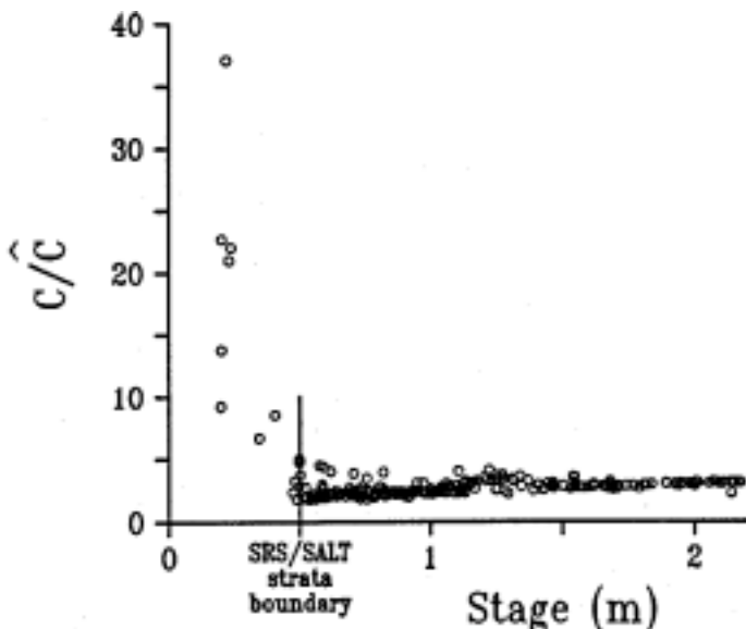
Figure 2-Ratio of measured to estimated suspended sediment concentration ( c/\hat{c} ) against stage for the North Fork of the Mad River near Korb, California (water year 1984). The boundary between the simple random sampling and the SALT (Selection At List Time) strata is indicated by the vertical line at about 0.5 m stage. Values of the ratio for stages above the boundary have nearly constant slope and are suitable for SALT sampling. Values less than the boundary stage are not constant and are sampled with simple random sampling.
