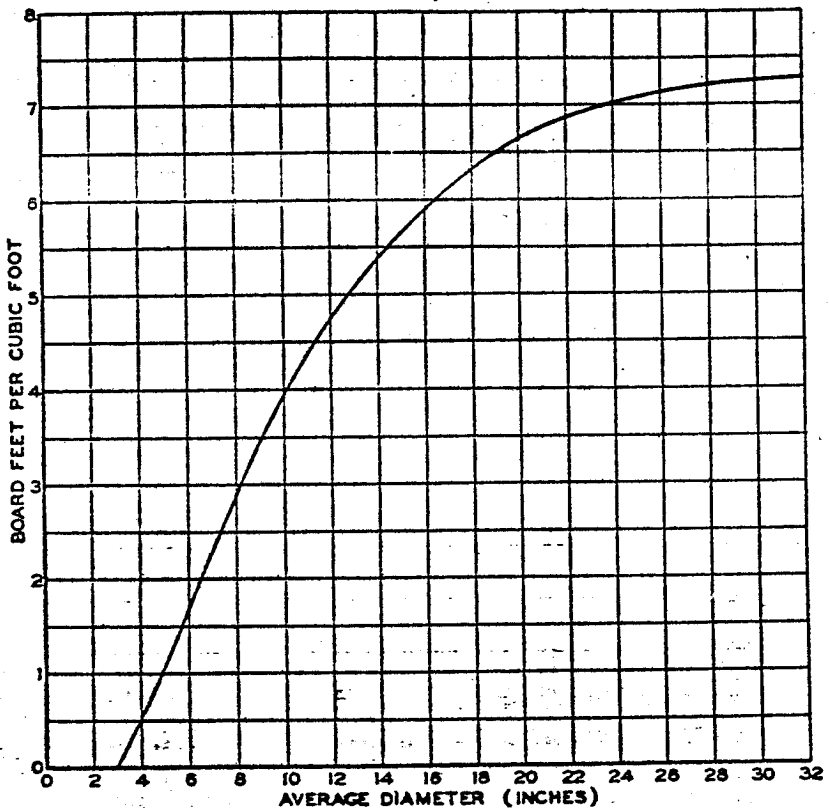
FIGURE 7.—The ratio of volume of stand in board feet to volume in cubic feet, in relation to average diameter of stand
