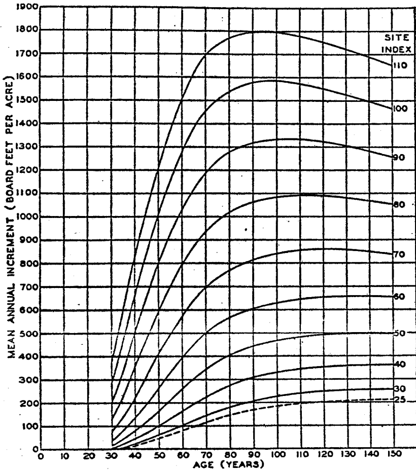
FIGURE 10.—Mean annual increment in board feet culminates at 95 years on the best sites and at 150 years and more on the poorest sites
