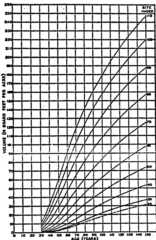
FIGURE 8.—Volume in board feet by the international rule (1/2-inch kerf), trees 8 inches and larger, average of well-stocked stands, average composition.
