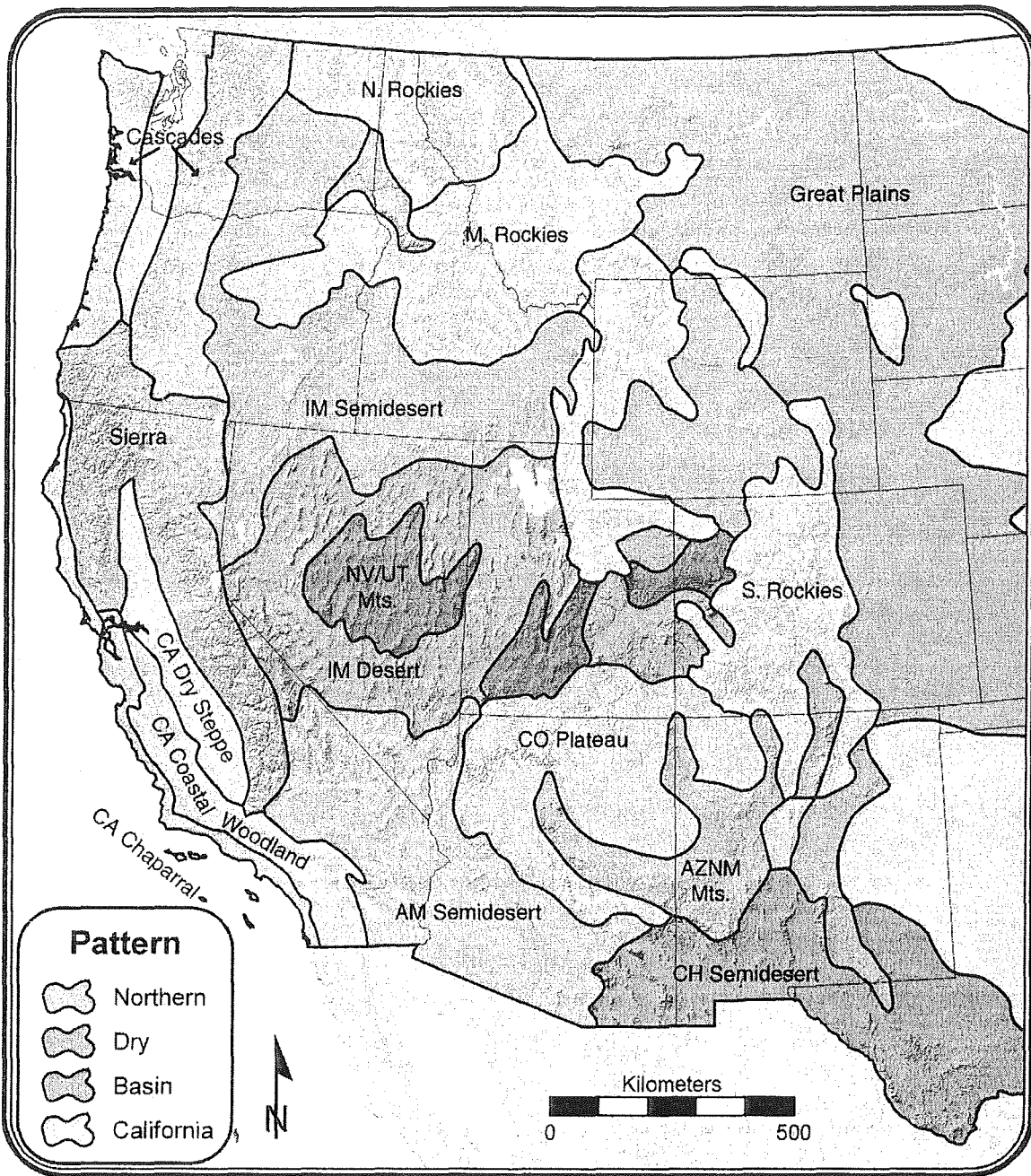
FIG. 2. Ecoprovinces of the western United States and common patterns of climate-fire associations from correlation and diagnostic regression models (see Results and Discussion). The 16 ecoprovinces for which we provide fire or fire/climate models are labeled. The similar colors group ecoprovinces with similar patterns of climate relationships (northern/mountain ecoprovinces, dry/lower-elevation ecoprovinces, Great Basin and Columbia Basin ecoprovinces, and California ecoprovinces). See Table 1 for an explanation of ecoprovince abbreviations.
