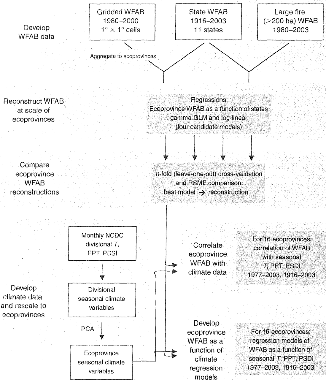
FIG. 3. Data handling and analysis workflow. Abbreviations are: GLM, generalized linear models; NCDC, National Climatic Data Center; PCA, principal components analysis; PSDI, Palmer drought severity index; PPT, precipitation; RMSE, root mean square error; T , temperature; WFAB, wildland fire area burned.
