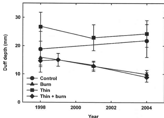
Fig. 4. Change in duff depth (mean \pm standard error) with four fuel reduction treatments in northeastern Oregon.
