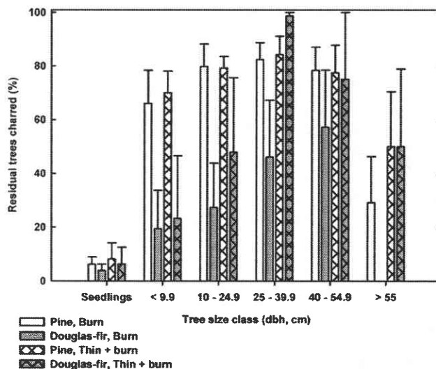
Fig. 5. Percentage of residual trees with bole charring (mean \pm standard error) by tree size and species after the burn and thin + burn treatments in northeastern Oregon.
