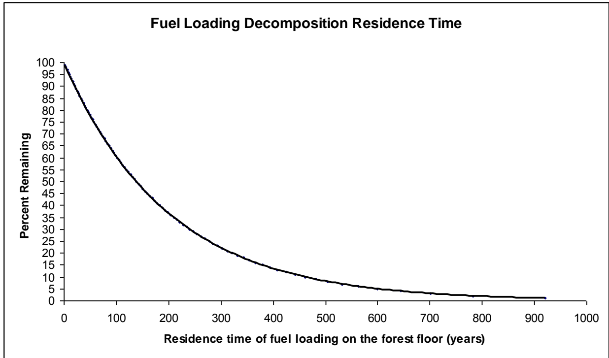
Fig. 5. Fuel loading residence time using Erickson et al. (1985) decomposition constant.
