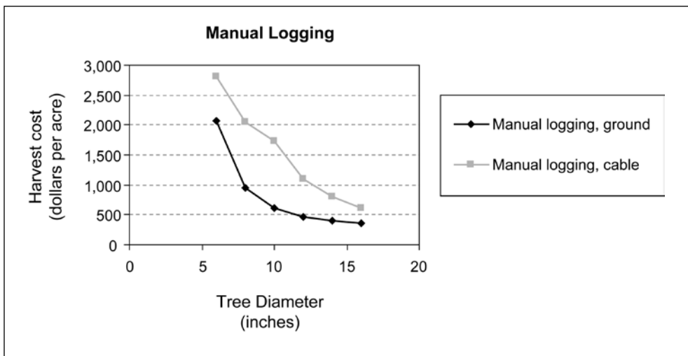
Figure 6—This comparison of the cost of a cable yarding system and a ground-based skidding system both with manual logging illustrates the cost disadvantage of harvesting where cable systems are required.
