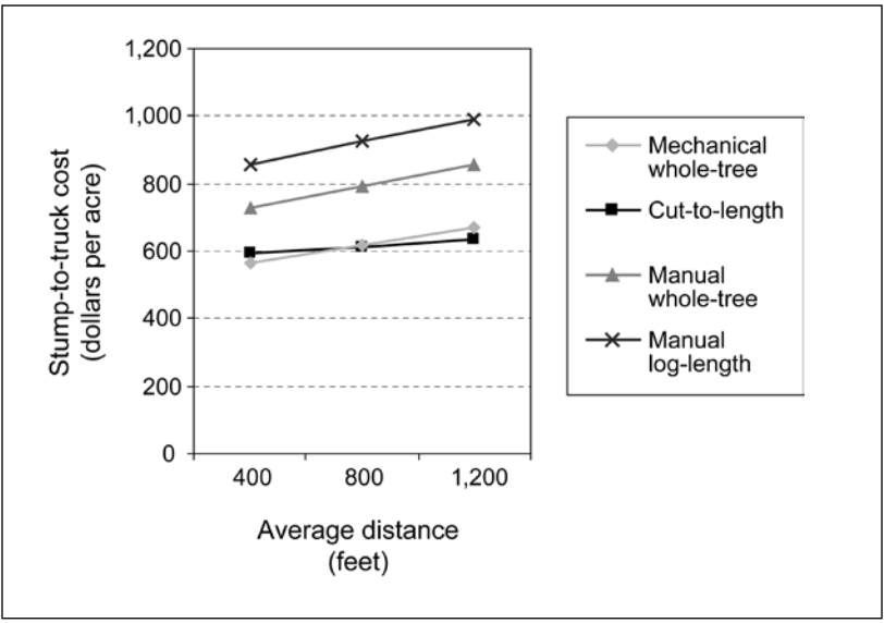
Figure 12—Stump-to-truck cost for ground-based systems harvesting 600 cubic feet per acre of 8-inch ponderosa pine on a 25-percent slope with skidding or forwarding distances of 400 to 1,200 ft.
