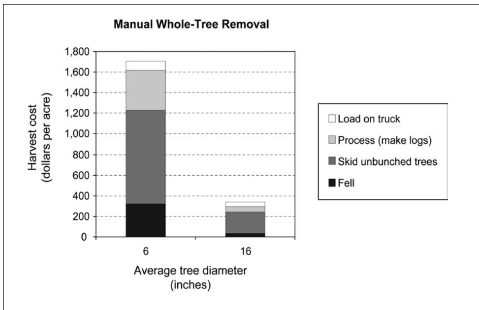
Figure 1—Cost of thinning 600 cubic feet per acre with manual felling and whole-tree skidding. When manual felling is used, the cost of removing smaller trees is higher in every step from the stump to the truck.
