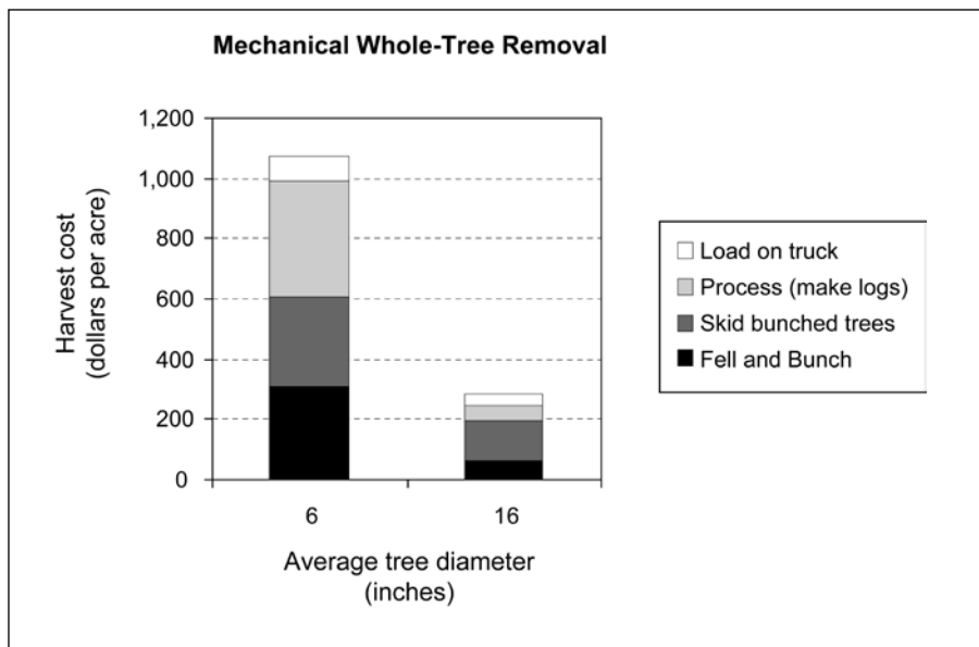
Figure 2—Cost of thinning 600 cubic feet per acre with mechanical felling and whole-tree skidding. Mechanical harvesting of trees reduces total cost, but the cost for smaller trees is still higher at every step from the stump to the truck.
