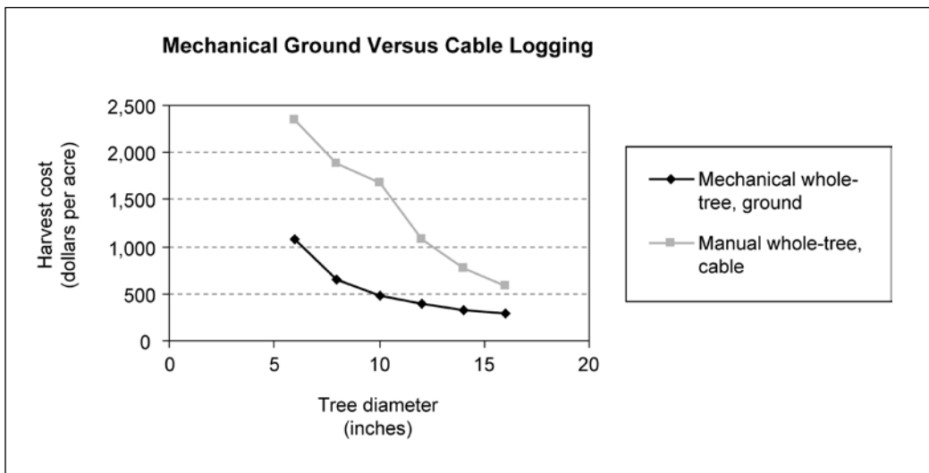
Figure 7—This comparison of harvesting cost for whole-tree logging with cable and ground-based systems illustrates the cost disadvantage of harvesting where cable systems are required. Cost differences are magnified, especially for small-diameter trees, when the ground-based system can use mechanical felling and whole-tree skidding.
