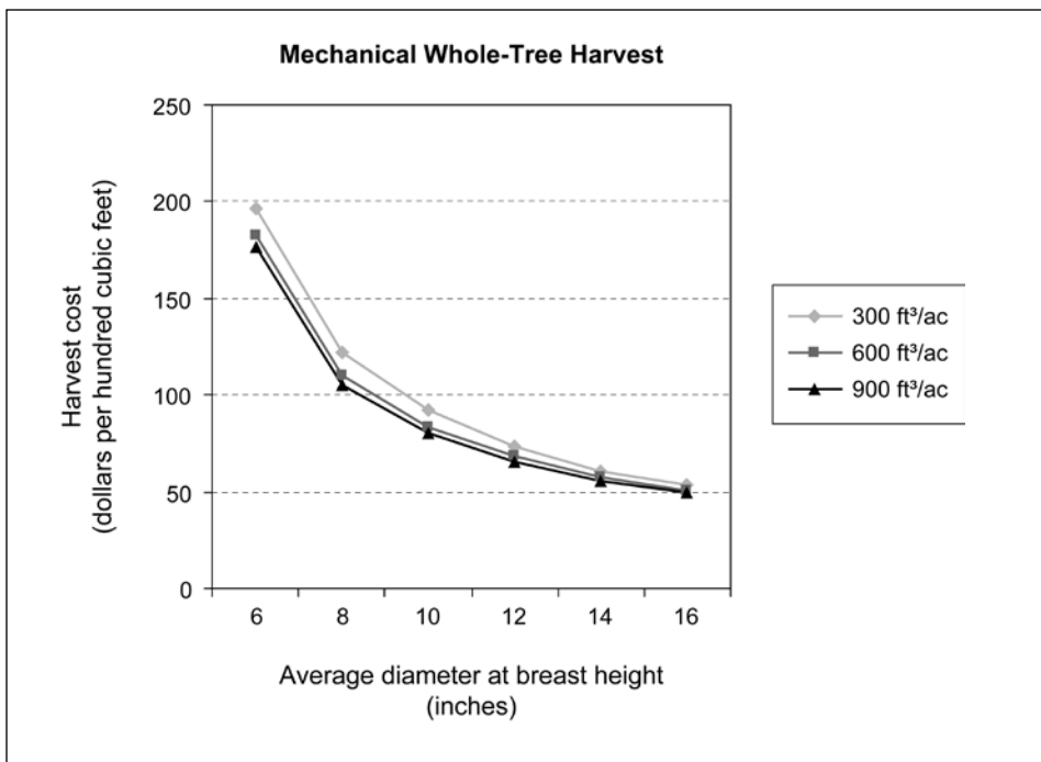
Figure 3—Cost of thinning with mechanical felling and whole-tree skidding with equipment move-in costs excluded. Volume per acre has little effect on harvesting cost when move-in costs are excluded.
