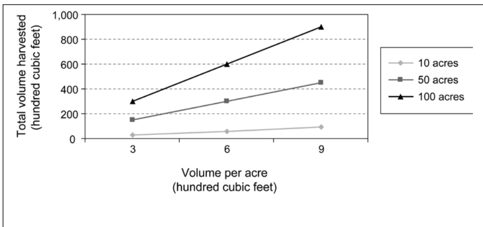
Figure 4—Total harvest volume for a range of volumes per acre and size of unit.
