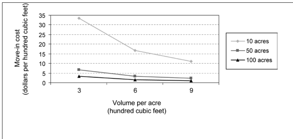
Figure 5—Contribution of move-in cost to total cost per hundred cubic feet for a range of volumes per acre and size of unit when move-in cost is $1,000. The cost of moving equipment to the site can be substantial for small isolated units.
