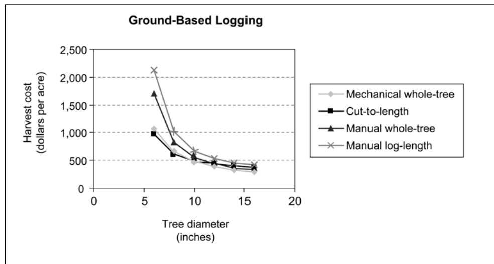
Figure 8—Harvesting costs for 600 cubic feet per acre for different types of ground-based harvesting systems. Notice that the differences are much greater for small-diameter trees than for larger trees.
