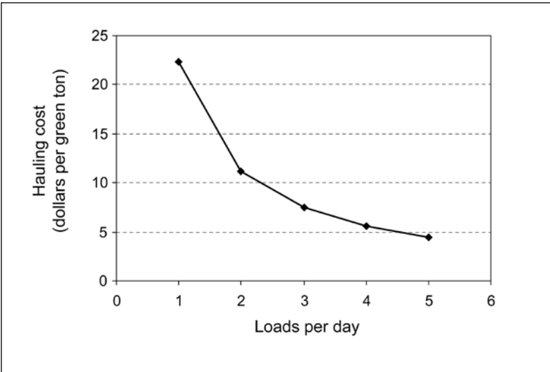
Figure 11—Hauling cost per green ton for a range of loads per day for a truck hauling 26 tons and costing $580 per day.
