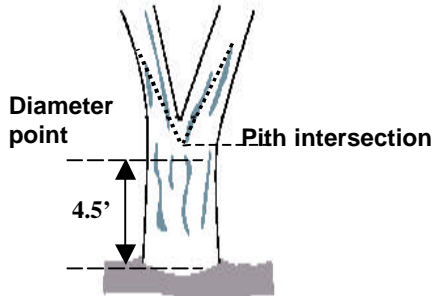
Figure 12. One tree
