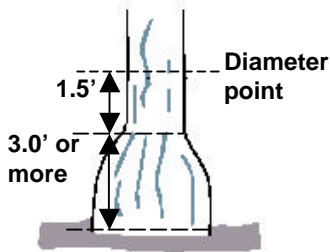
Figure 14. Bottleneck tree
