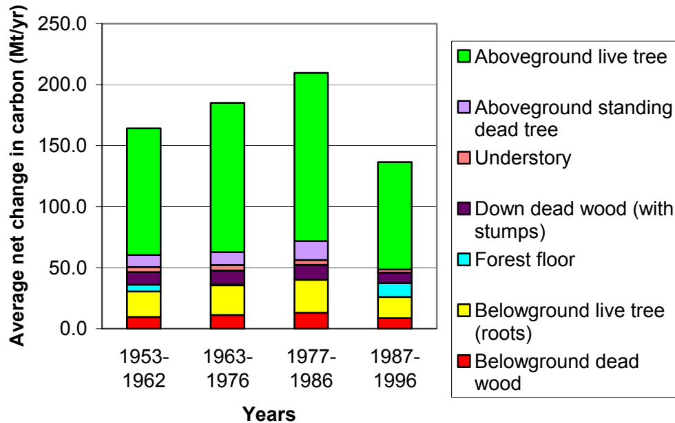
Figure 27.1—Average annual net change in forest ecosystem non-soil carbon pools (Mt/yr) for all forest land of the conterminous United States, 1953-1996. All net carbon stock changes are positive, indicating absorption of carbon by the forest from the atmosphere. The only emission of carbon (-1.7 Mt/yr) occurred for aboveground standing dead trees carbon in 1987-1996.
