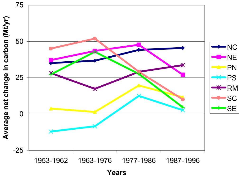
Figure 27.3—Average annual net change in non-soil forest ecosystem carbon (Mt/yr) by region of the conterminous United States, 1953-1996. (NC=North Central, NE=Northeast, PN=Pacific Northwest, PS=Pacific Southwest, RM=Rocky Mountain, SC=South Central, SE=Southeast. Regions are the same as in Smith and others (2001), with the exception of the States of ND, eastern SD, NE, and KS, which are compiled with the NC region.
