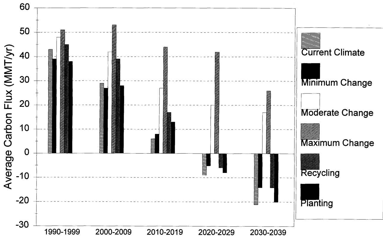
Figure 2.—Carbon flux for baseline, two alternative carbon sequestration scenarios, and three climate change scenarios.
