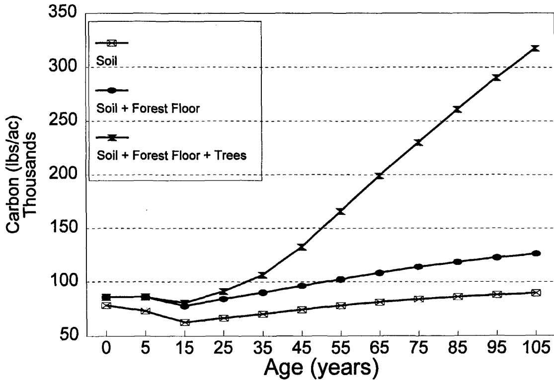
Figure 1.—Carbon changes over time for average Douglas-fir stands in the northern Rocky Mountains.
