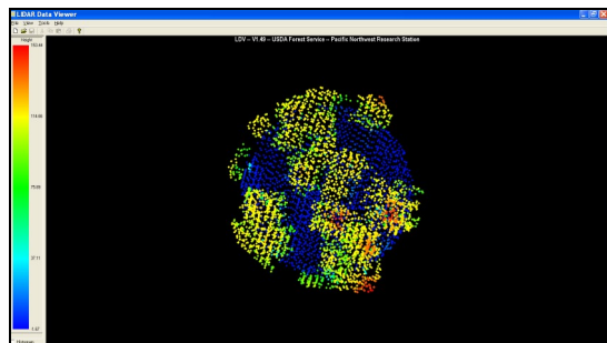
Overhead view of the sample lidar point cloud subset.
